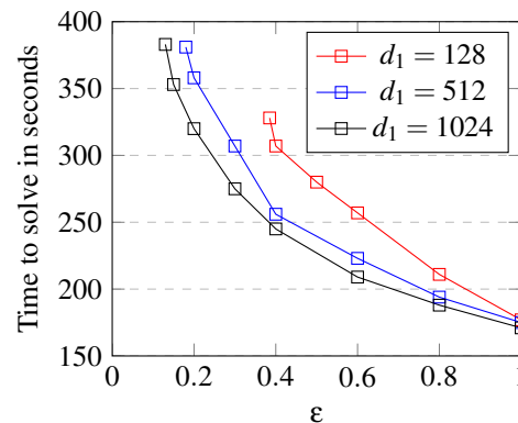
Figure 9: Computation time to solve the SparsePIR linear system vs \epsilon on 2^{20} elements for dimension sizes d_1 = 128, 512 and 1024 . The graphs suggest that the \epsilon lower bounds for d_1 = 128, 512 and 1024 are roughly 0.38, 0.18, and 0.13 respectively. We chose band parameter w \in [50, 60] .
