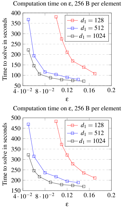
Figure 10: Computation time to solve the SparsePIR g linear system vs \epsilon on 2^{20} elements for dimension sizes d_1 = 128, 512 and 1024 . We chose band parameter w \in [85, 120] .
