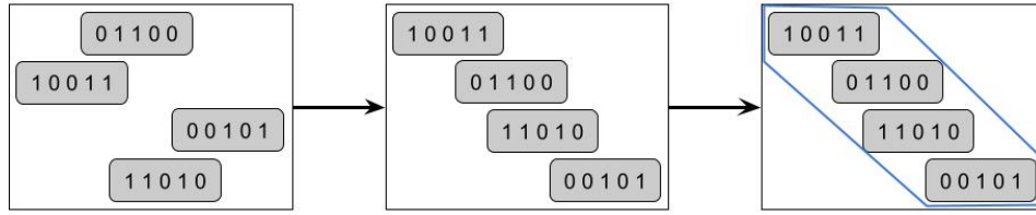
Figure 4: The left matrix is a random band matrix with 4 rows and band width w = 5 . The middle matrix is the intermediate step of the Gaussian elimination that sorts rows by band location. The final matrix shows that Gaussian elimination only considers a small subset of entries.
