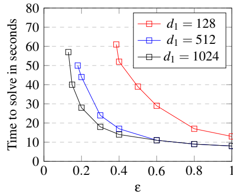
Computation time on \epsilon , 16 KB per element
